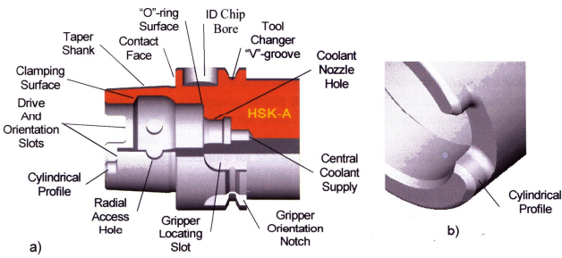
Fig. 4.2. Basic Features of an HSK Shank, Type A a) – cutaway view, b) – cylindrical profile of drive slots
