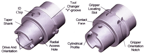
Fig. 4.1. An overview of an HSK Shank Type A
