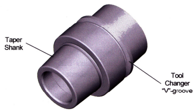
Fig. 4.9. An overview of an HSK Shank, Type E
