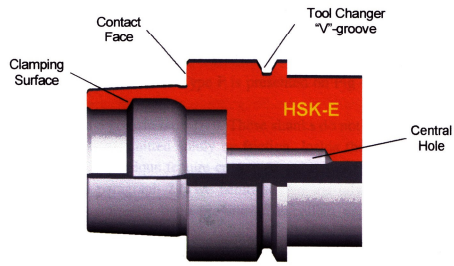
Fig. 4.10. Cutaway view of an HSK Shank, Type E
