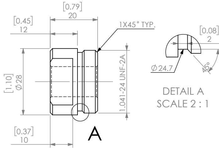
570-ADJ head
