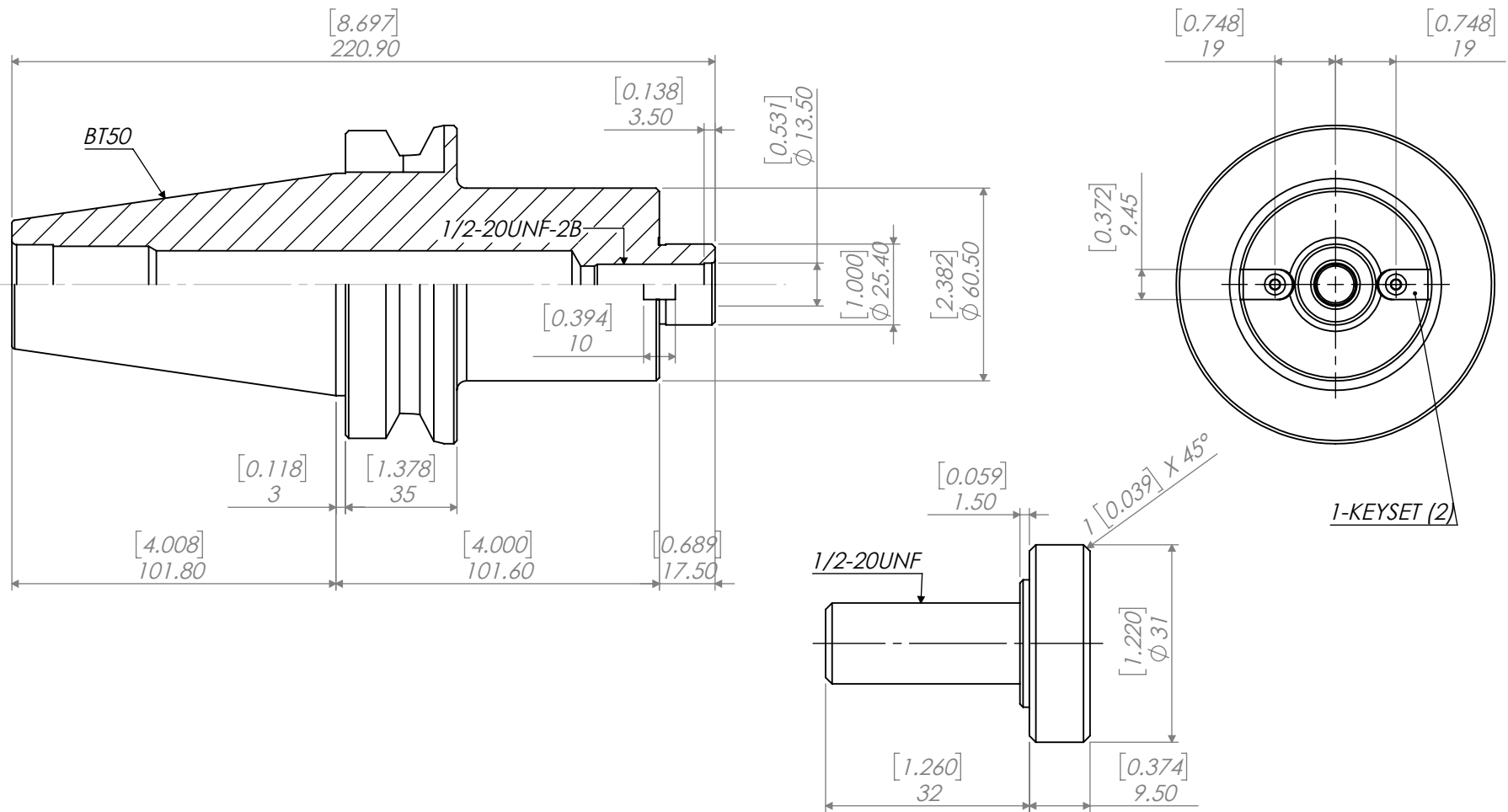
ARBOR SCREW (1:1)
