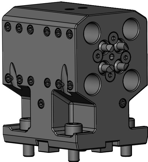
90 DEGREE STATIC TOOL OUTPUT: 3/4" BORING BAR MAIN & SUB QUAD COOLANT: EXTERNAL
