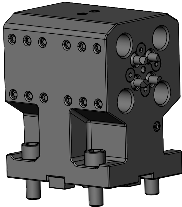
90 DEGREE STATIC TOOL OUTPUT: 3/4" BORING BAR MAIN & SUB QUAD COOLANT: EXTERNAL
