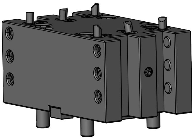
STRAIGHT STATIC TOOL OUTPUT: 3/4" SQR SHANK MAIN & SUB DUAL COOLANT: EXTERNAL
