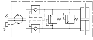
Internal Schematic
