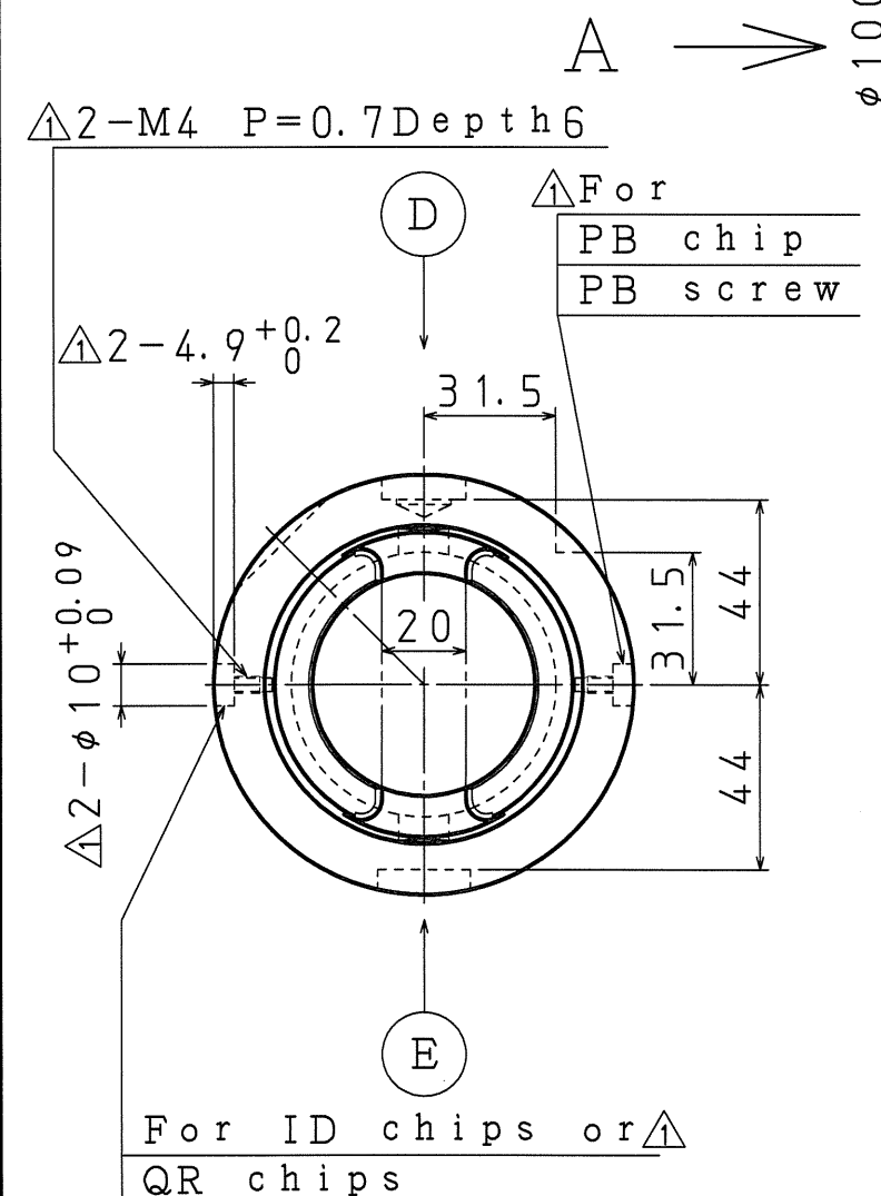
VIEW A (S=1:2)
