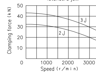
Clamping force characteristic diagram (Standard jaw)
