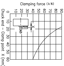
Static clamping force characteristic diagram
