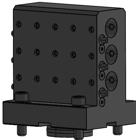
90 DEGREE STATIC TOOL OUTPUT: 1" BORING BAR MAIN & SUB TRIPLE COOLANT: EXTERNAL
