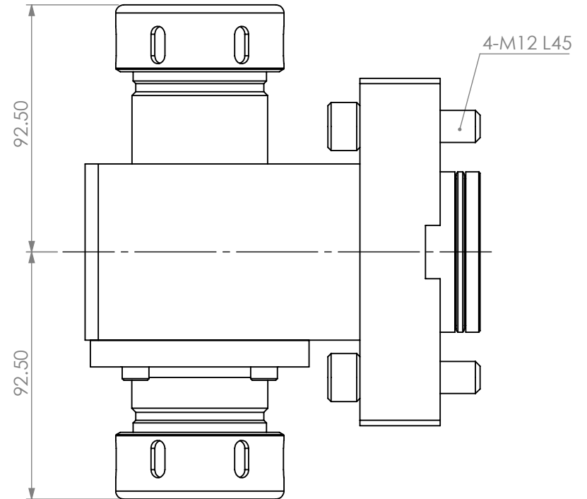
90 DEGREE STATIC TOOL OUTPUT: ER40 MAIN & SUB COOLANT: EXTERNAL & INTERNAL
