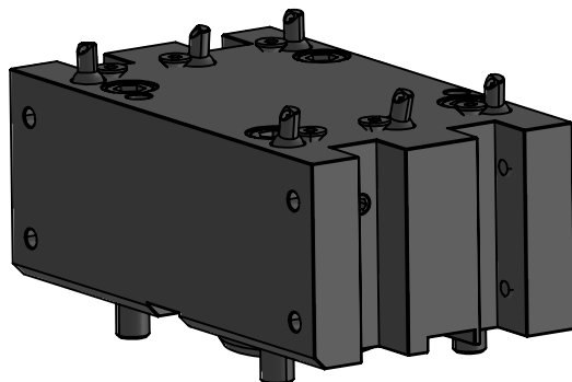
STRAIGHT STATIC TOOL OUTPUT: 3/4" SQR SHANK MAIN & SUB DUAL COOLANT: EXTERNAL
