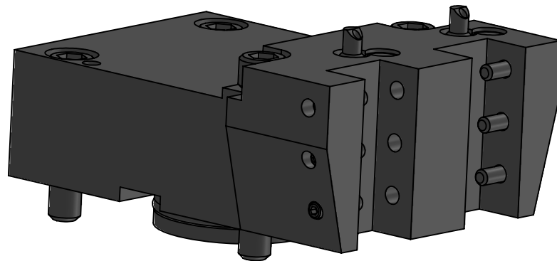
STRAIGHT STATIC OUTPUT: 3/4" SQR SHANK DUAL Y-AXIS COOLANT: EXTERNAL
