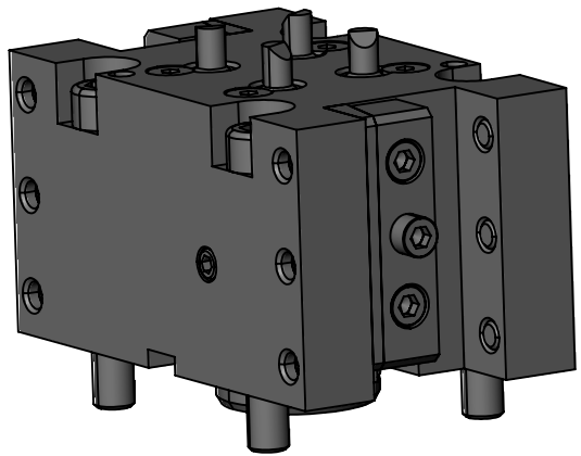
STRAIGHT STATIC TOOL OUTPUT: 3/4" SQR SHANK MAIN & SUB COOLANT: EXTERNAL **WEDGE CLAMP MOVABLE LEFT/RIGHT**
