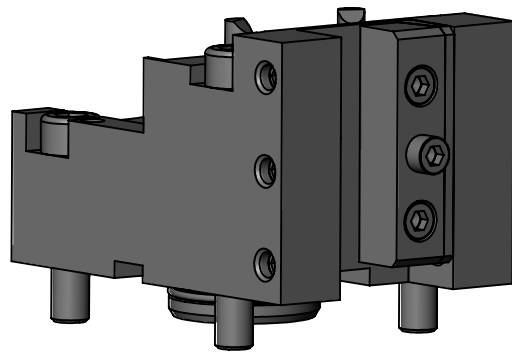
STRAIGHT STATIC TOOL OUTPUT: 3/4" SQR SHANK COOLANT: EXTERNAL **WEDGE CLAMP MOVABLE LEFT/RIGHT**
