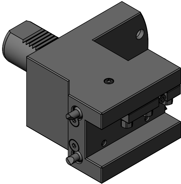
90 DEGREE VDI40 STATIC TOOL OUTPUT: 20mm SQR SHANK COOLANT: EXTERNAL **WEDGE CLAMP MOVABLE LEFT/RIGHT**
