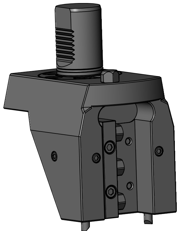
STRAIGHT VDI40 STATIC TOOL OUTPUT: 1" SQR SHANK COOLANT: EXTERNAL **WEDGE CLAMP MOVABLE LEFT/RIGHT**
