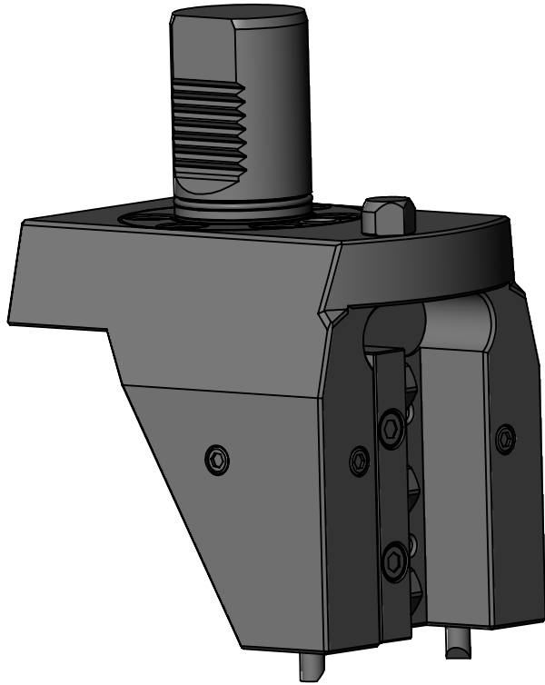
STRAIGHT VDI40 STATIC TOOL OUTPUT: 25mm SQR SHANK COOLANT: EXTERNAL **WEDGE CLAMP MOVABLE LEFT/RIGHT**
