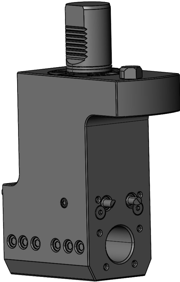
90 DEGREE VDI40 STATIC TOOL OUTPUT: 1.1/4" BORING BAR MAIN & SUB COOLANT: EXTERNAL & INTERNAL **BACK PLATE REMOVABLE**
