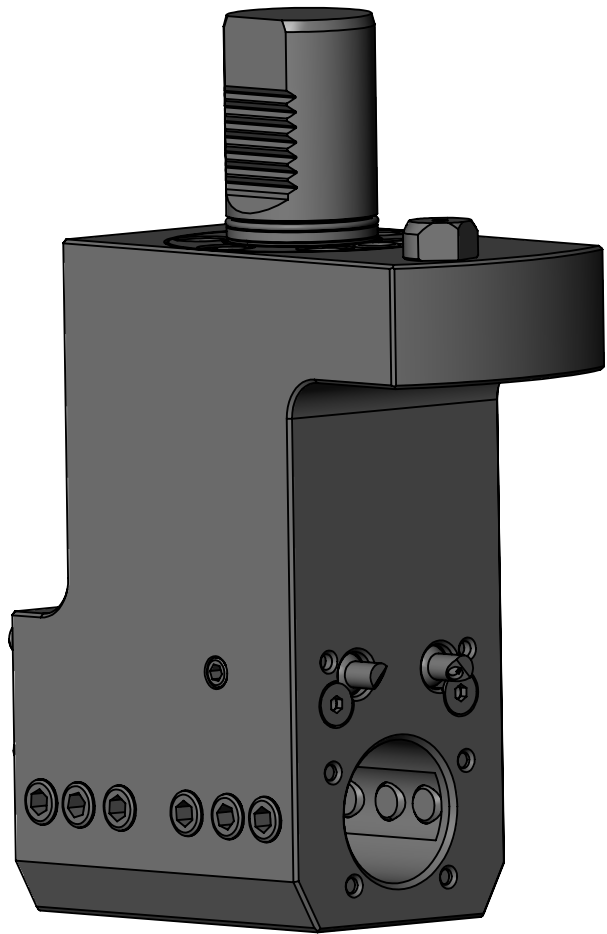
90 DEGREE VDI40 STATIC TOOL OUTPUT: 1.1/2" BORING BAR MAIN & SUB COOLANT: EXTERNAL & INTERNAL **BACK PLATE REMOVABLE**
