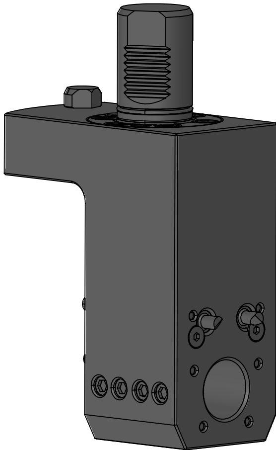
90 DEGREE STATIC TOOL OUTPUT: 1.1/4" BORING BAR COOLANT: EXTERNAL & INTERNAL **BACK PLATE REMOVABLE**
