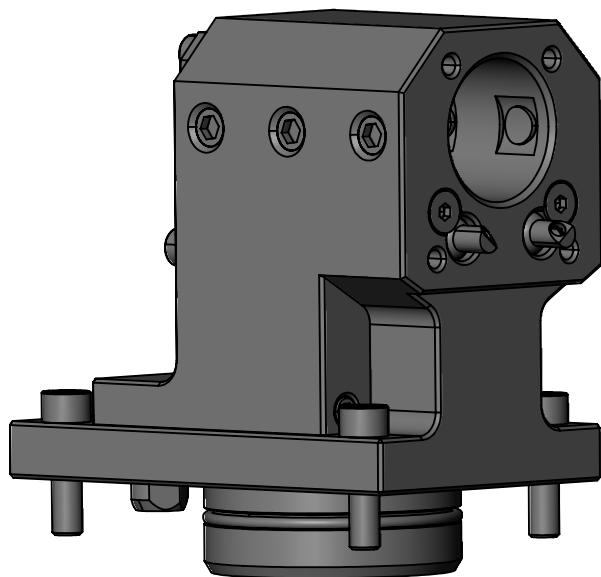
90 DEGREE STATIC TOOL OUTPUT: 1.1/2" BORING BAR COOLANT: EXTERNAL & INTERNAL **BACK PLATE REMOVABLE**
