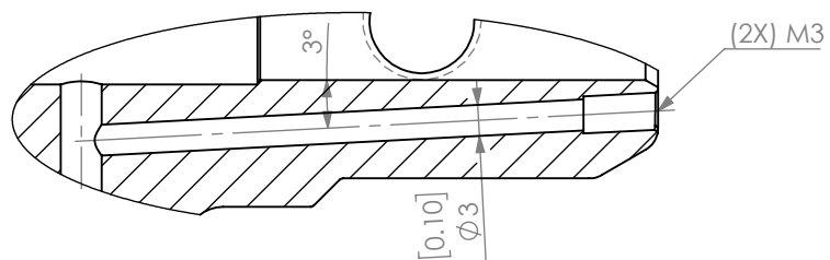
DETAIL A SCALE 1.5:1
