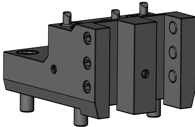
STRAIGHT STATIC TOOL OUTPUT: 1" SQR SHANK DUAL Y-AXIS COOLANT: EXTERNAL
