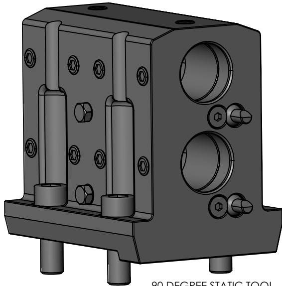
90 DEGREE STATIC TOOL OUTPUT: 1.1/4" BORING BAR MAIN & SUB DUAL COOLANT: EXTERNAL
