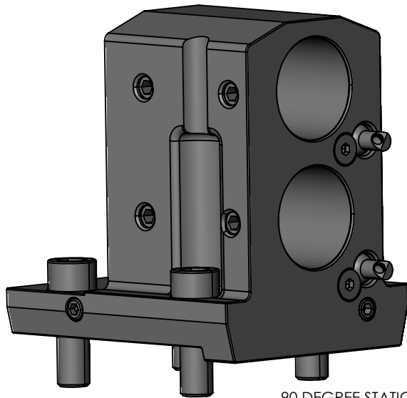
90 DEGREE STATIC TOOL OUTPUT: 1.1/2" BORING BAR DUAL COOLANT: EXTERNAL
