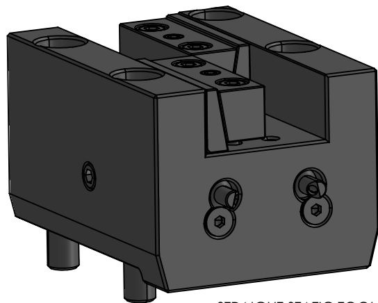
STRAIGHT STATIC TOOL OUTPUT: 1" SQR SHANK MAIN & SUB COOLANT: EXTERNAL **WEDGE CLAMP MOVABLE LEFT/RIGHT**
