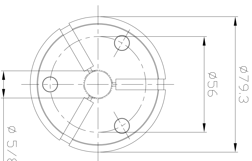
Serrated hole
