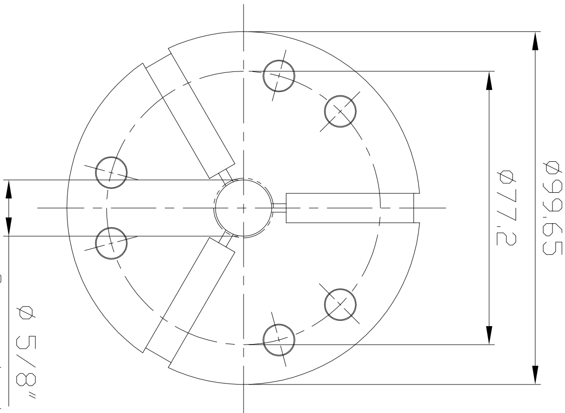
Serrated hole
