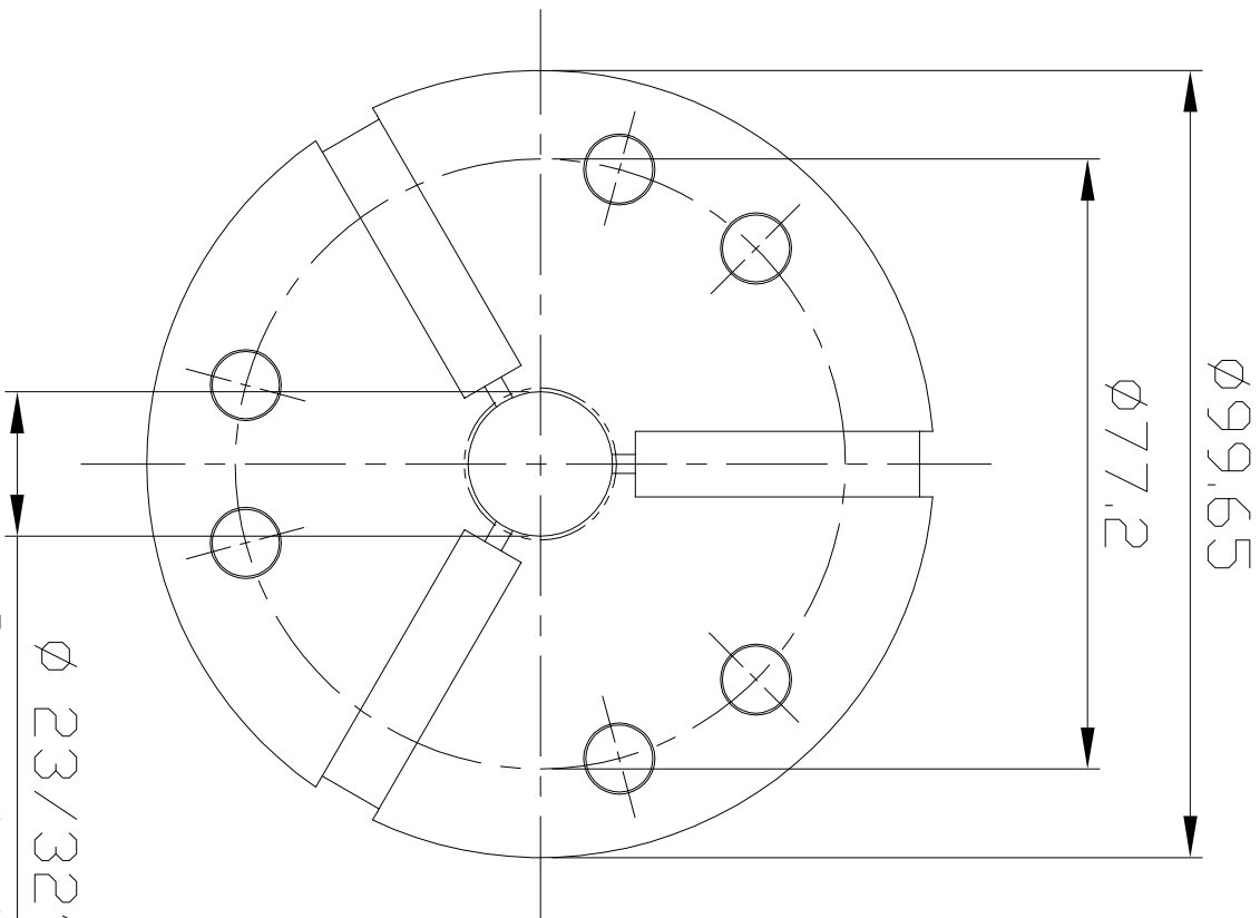
Serrated hole
